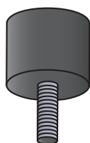
Vibration-proof buffer Ø 20 Vibration-proof buffer Ø 0,787' COD. BFAMMO20X15M6X16*45
