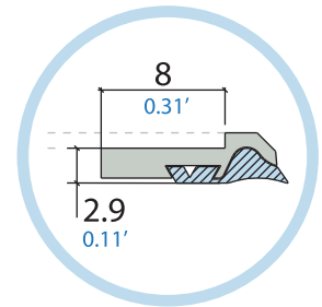
Metal-jacketed rubber wiper MGRA0006 COD.
