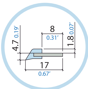
Non-jacketed wiper COD. BFRASCA6L1MT-000
